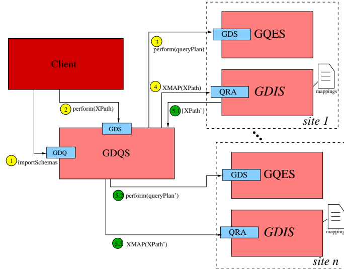
Figure 1. Data integration-enabled query processing on the Grid: service interactions.
