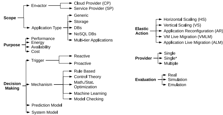
Fig. 1: Classification Scheme
